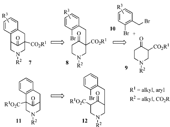
Figure 2. Synthetic strategy towards benzomorphan based on an intramolecular Buchwald–Hartwig arylation.
