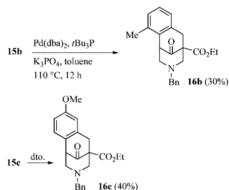
Scheme 4. Palladium-catalyzed intramolecular ketone arylation to yield the benzomorphan derivatives 16b and 16c .
