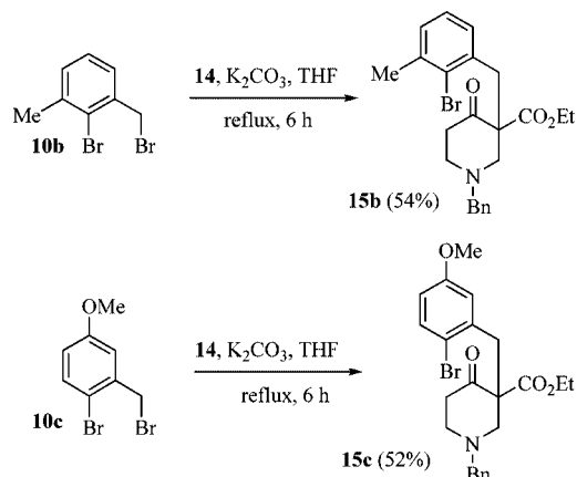
Scheme 3. Alkylation of ethyl 1-benzyl-4-oxopiperidine-3-carboxylate ( 14 ) with benzyl bromides 10b and 10c .
