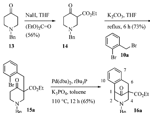
Scheme 1. Alkylation of ethyl 1-benzyl-4-oxopiperidine-3-carboxylate ( 14 ) and palladium-catalyzed intramolecular ketone arylation of 15a to yield the benzomorphan derivative 16a .
