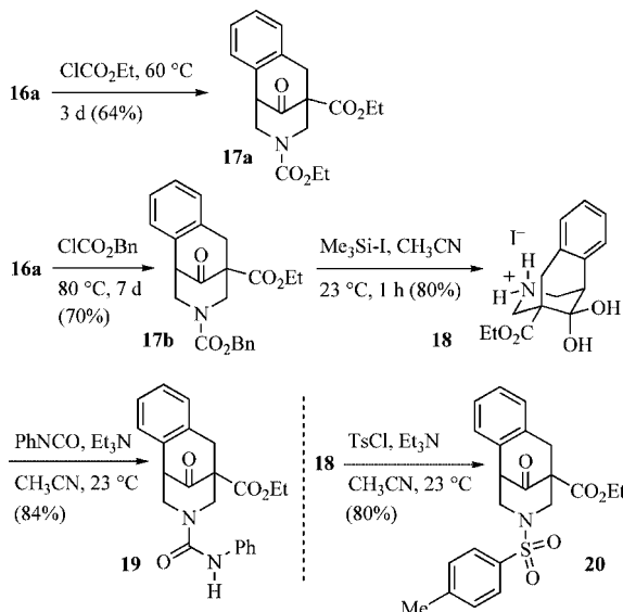
Scheme 2. Conversion of the N -benzyl compound 16a to the urethanes 17a and 17b . Cleavage of the Cbz group to yield the ammonium iodide 18 followed by derivatization reactions on the tricyclic amino ketone.
