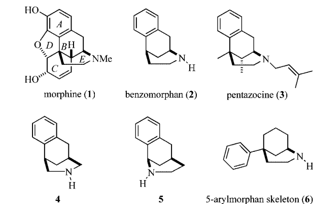
Figure 1. Structures of morphine ( 1 ), and prominent analogs derived from it.
