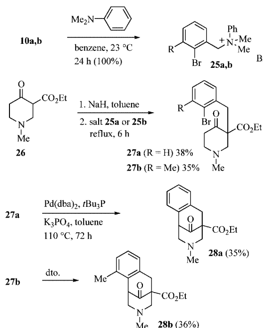
Scheme 6. Alkylation of the N -methyl piperidone 26 with the ammonium salts 25a and 25b followed by cyclization to the N -methyl-substituted benzomorphan derivatives 28a and 28b .
