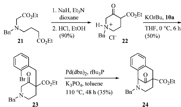
Scheme 5. Synthesis of ethyl 1-benzyl-3-oxopiperidine-4-carboxylate ( 23 ) and its Pd-catalyzed cyclization to 24 .
