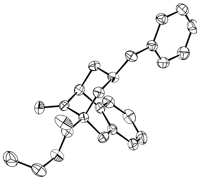
Figure 3. X-ray structure of benzomorphan 16a . The crystal sample was obtained by crystallization from hot heptane.
